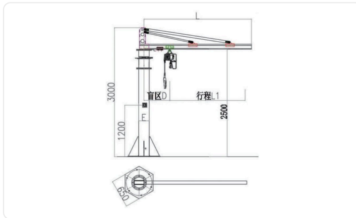
Aluminum Alloy Crane Dimension Drawing
